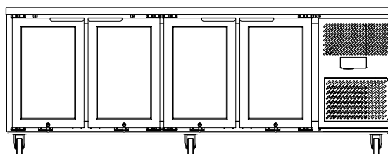
4 x Glass Doors AXR.UCGN.4G 164kg 0°C - 6°C 230VAC / 10A
