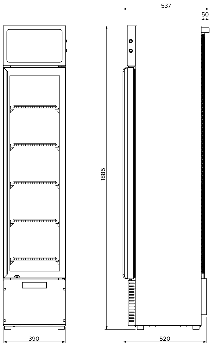
FRONT VIEW
