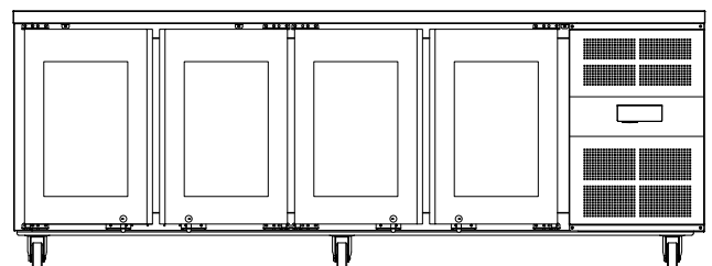
4 x Glass Doors AXR.UCGN.4G 164kg 0°C - 6°C 230VAC / 10A
