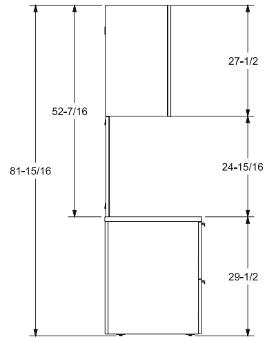
TYPICAL 2-HIGH SIDE PROFILE
