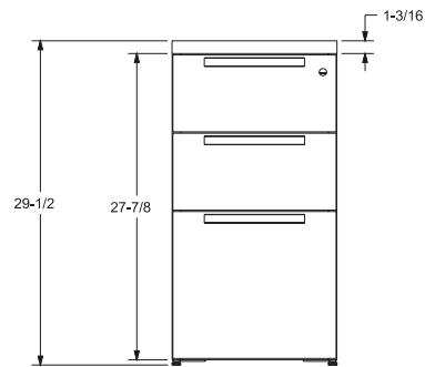
PEDESTAL FRONT PROFILE
