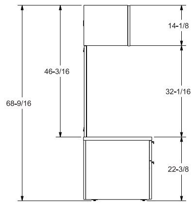
TYPICAL 1-HIGH SIDE PROFILE
