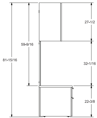
TYPICAL 2-HIGH SIDE PROFILE
