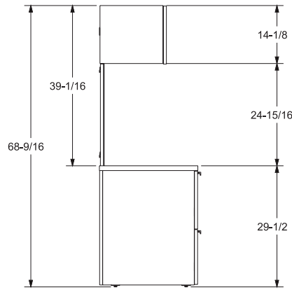
TYPICAL 1-HIGH SIDE PROFILE
