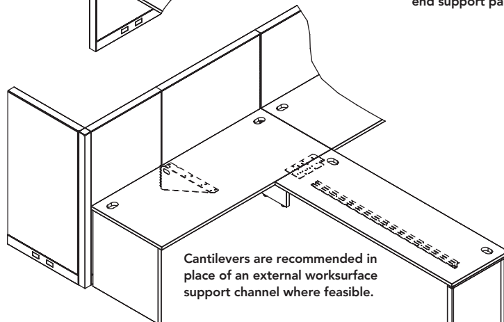
Worksurface runs 60"W or greater require an external worksurface support channel when a center support cantilever cannot be used. It is recommended for spans greater than 48"W. See pages 200 and 211.
