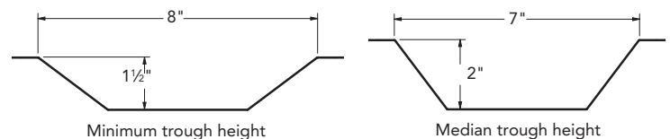
Cross-sectional Area Inside Under Worksurface Troughs
