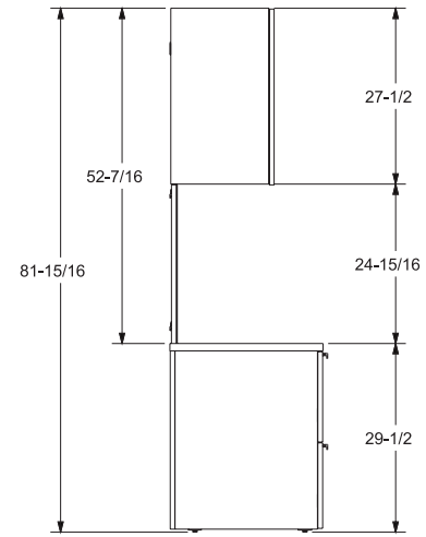
TYPICAL 2-HIGH SIDE PROFILE
