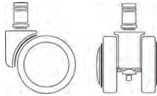
(B) Soft Wheel Wheel Diameter 2"
