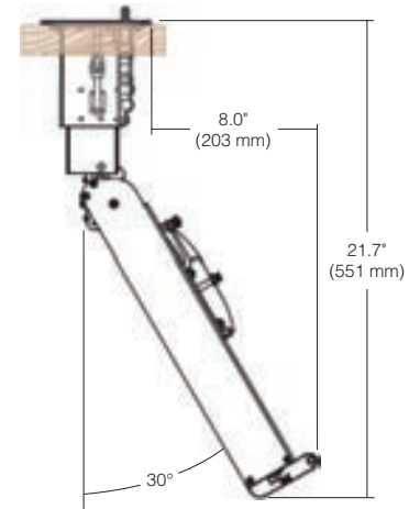
Angular Mounting
