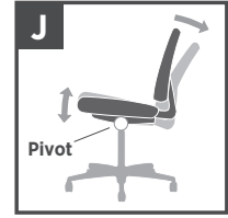
J. Synchro-tilt — Back reclines at a 2-to-1 ratio to seat angle. Allows user to recline while keeping seat cushion relatively level to floor.
