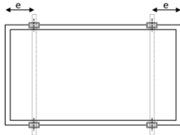
Fig. A2: Clamp position on long frames Mounting rails perpendicular to the longer frame
