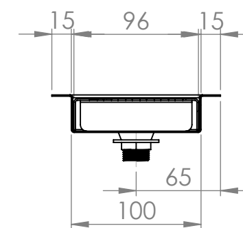
SECTION C-C
