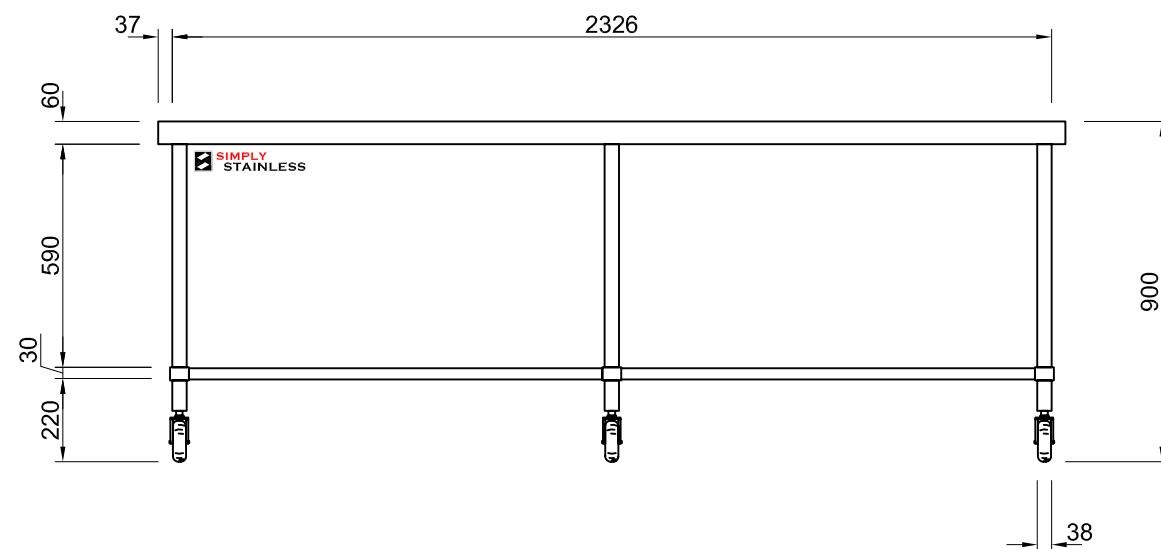
FRONT ELEVATION
