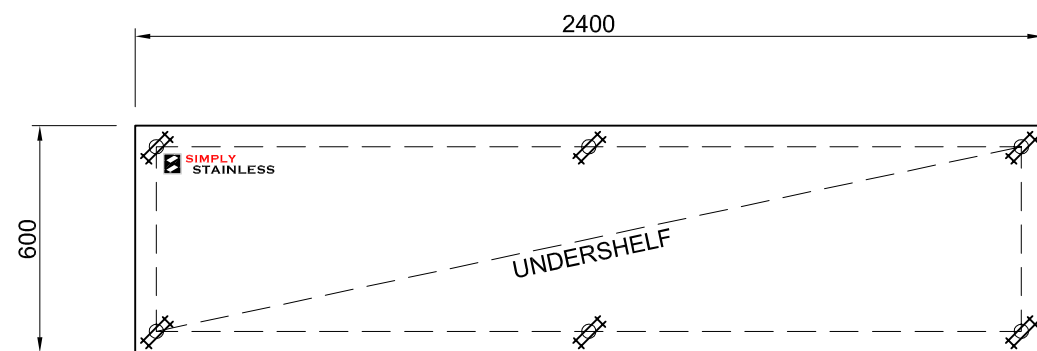
PLAN
