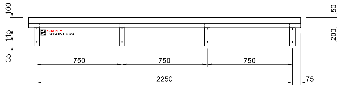
FRONT ELEVATION
