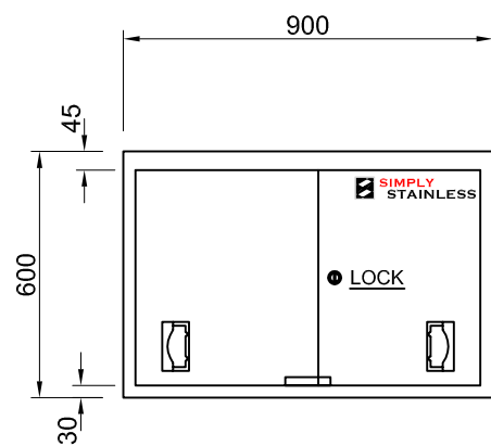
FRONT ELEVATION
