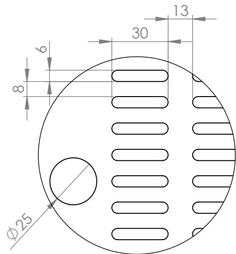
DETAIL C
