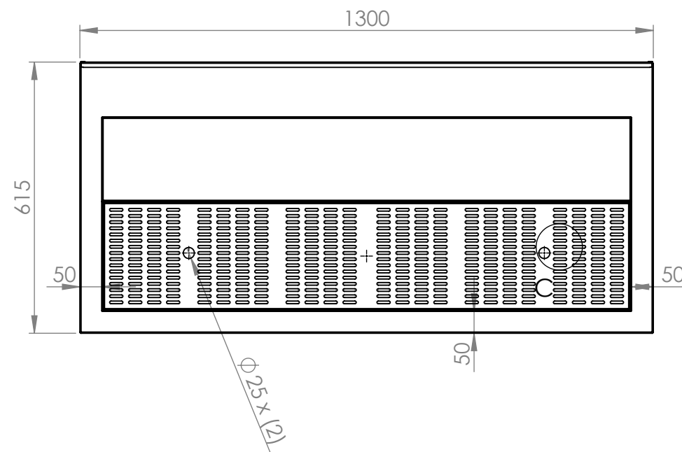
DETAIL B
