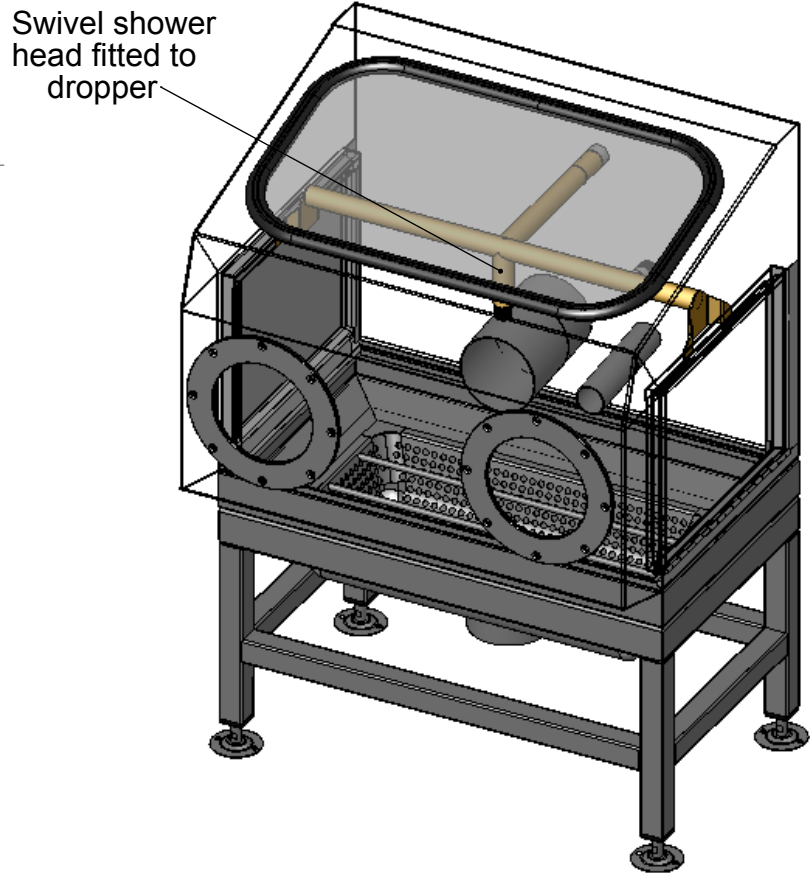
INTERNAL ISOMETRIC VIEW
