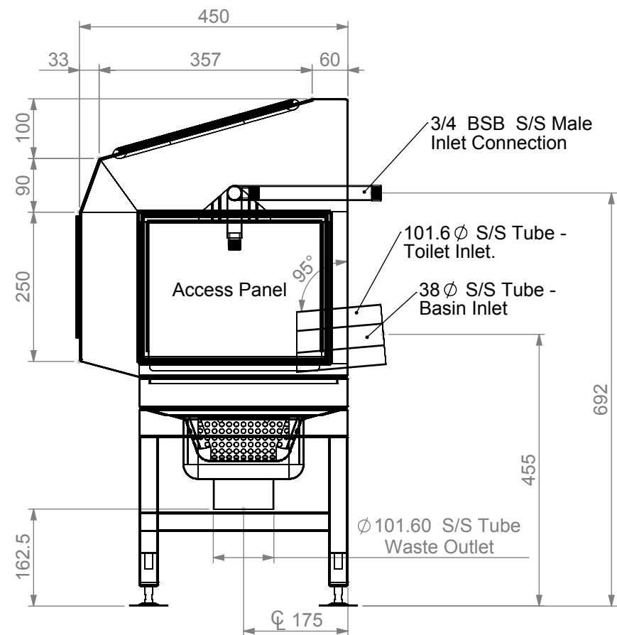
END VIEW
