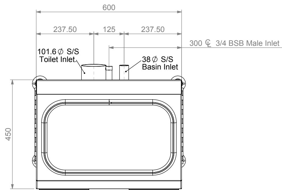
PLAN VIEW
