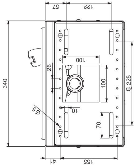
REAR VIEW
