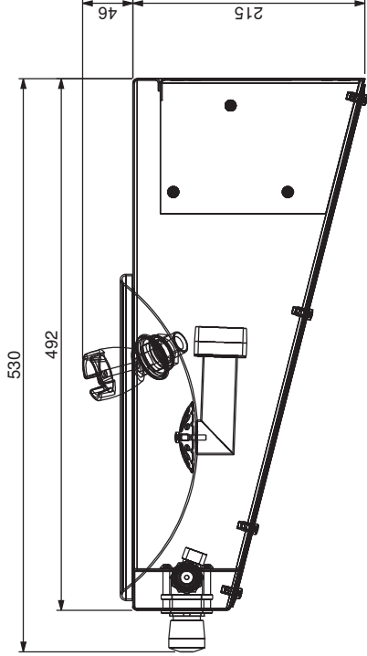
END VIEW
