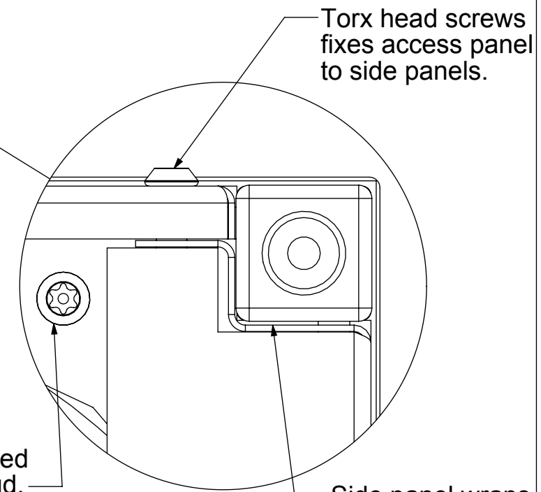
DETAIL I SCALE 1 : 1
