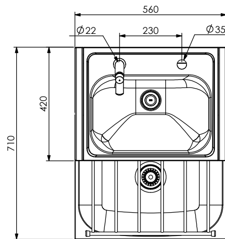
PLAN VIEW (Manual Tapware)
