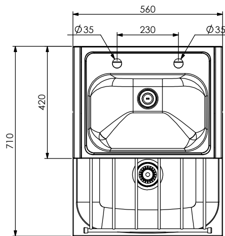
PLAN VIEW (Sensor Tapware)
