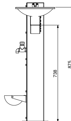
END VIEW
