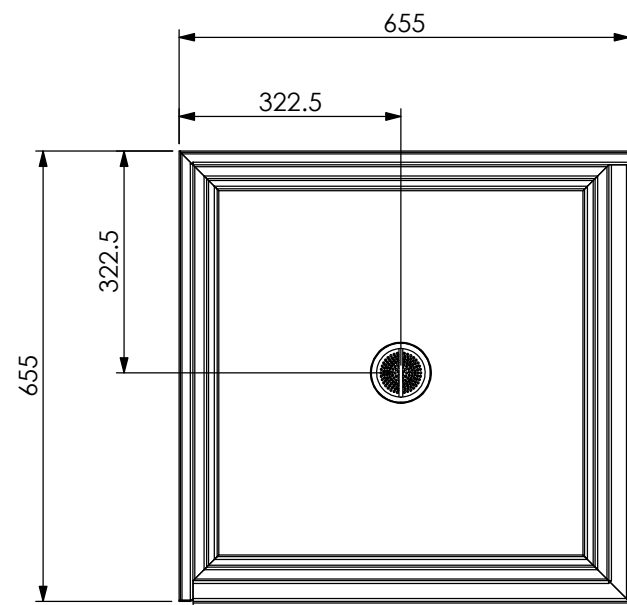
PLAN VIEW (Without grate & basket)
