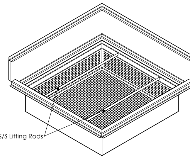
ISOMETRIC VIEW (Without Grate)
