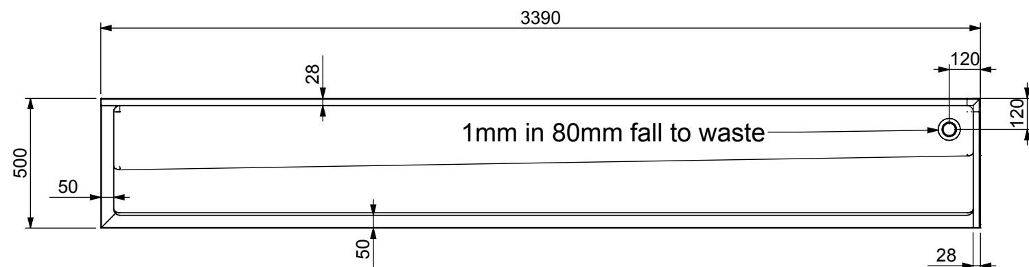
PLAN VIEW
