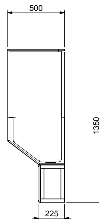
END VIEW
