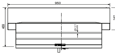
FRONT ELEVATION
