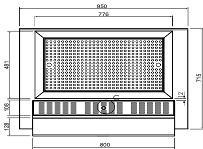
PLAN - LARGE ICE WELL
