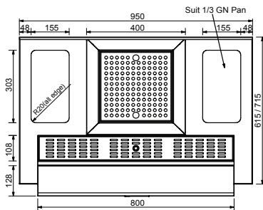
PLAN - SMALL ICE WELL
