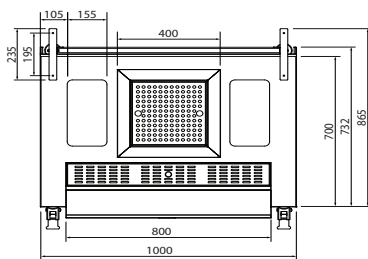
MOBILE ICE WELL- PLAN
