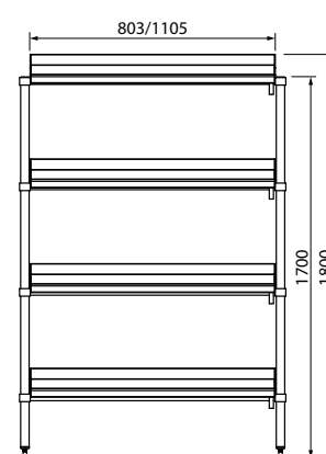
SS17.DF.0900 SIDE ELEVATION
