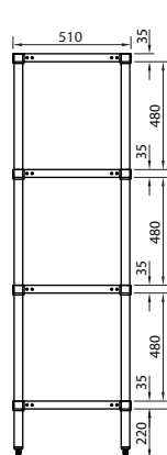
SS17.xxx SIDE ELEVATION
