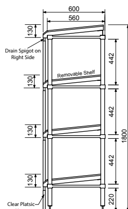
SS17.DF.xxx SIDE ELEVATION
