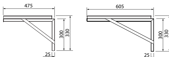
SIDE ELEVATION
