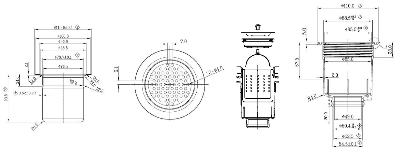
SECTION VIEW
