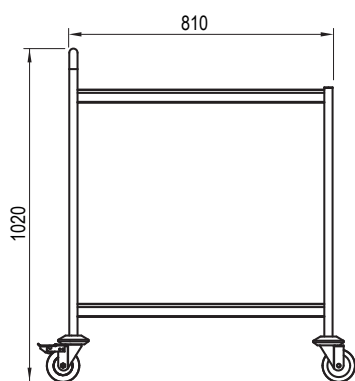
SS14 SIDE ELEVATION
