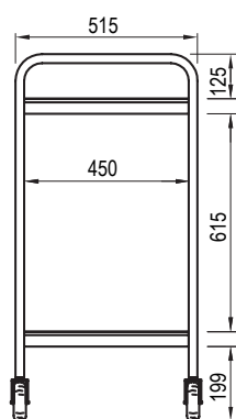
SS14 FRONT ELEVATION
