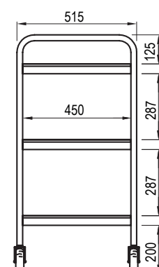
SS15 FRONT ELEVATION
