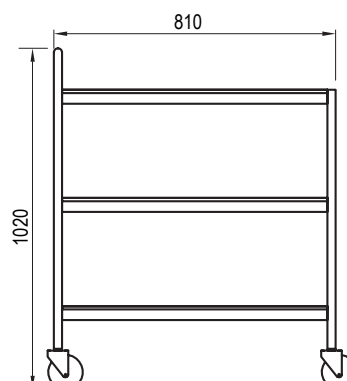
SS15 SIDE ELEVATION
