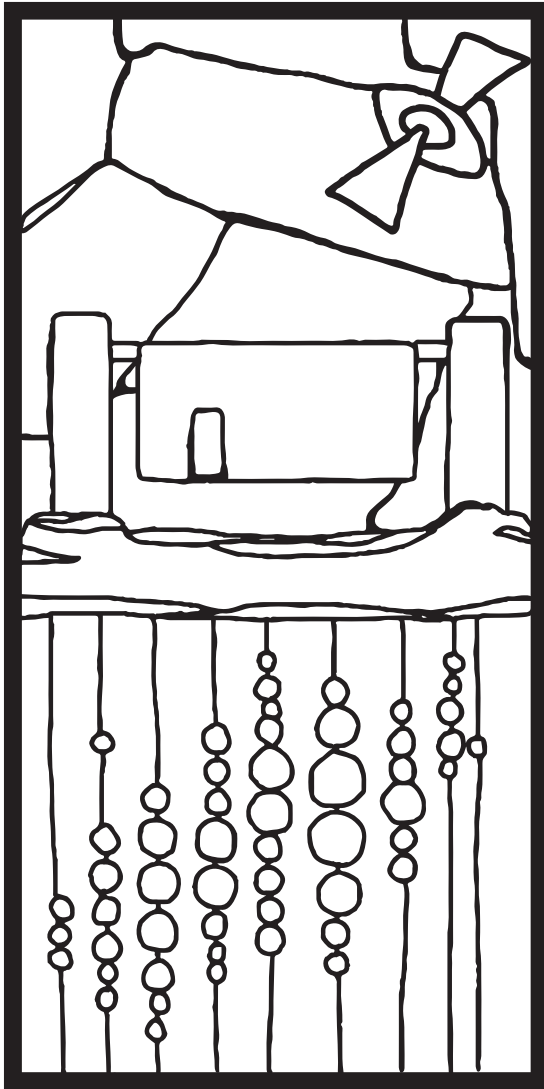
IceCube Neutrino Observatory (neutrinos)
