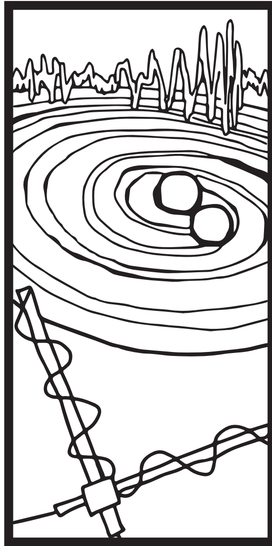
LIGO (gravitational waves)
