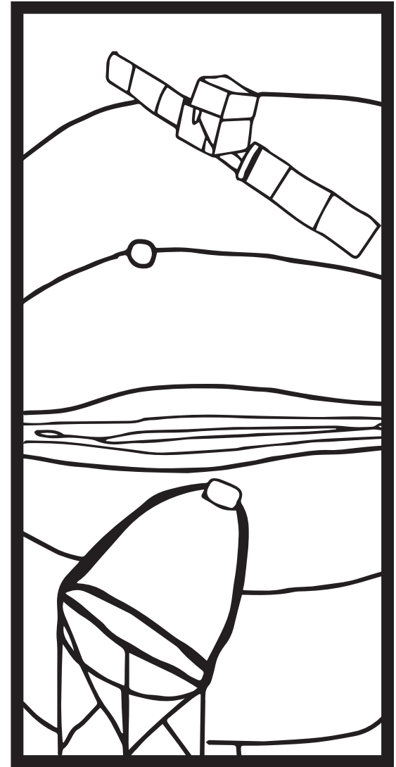
Fermi Space Telescope and MAGIC (gamma rays)
