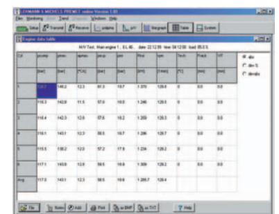
Engine data table
