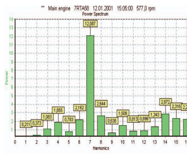
Torsional vibration spectrum
