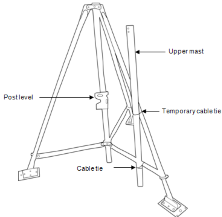
Figure 45: Upper mast (temporary)
