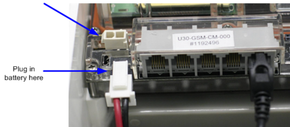
Figure 9: Connecting the Battery
