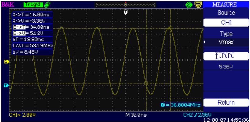
Figure 50 - Auto Mode
