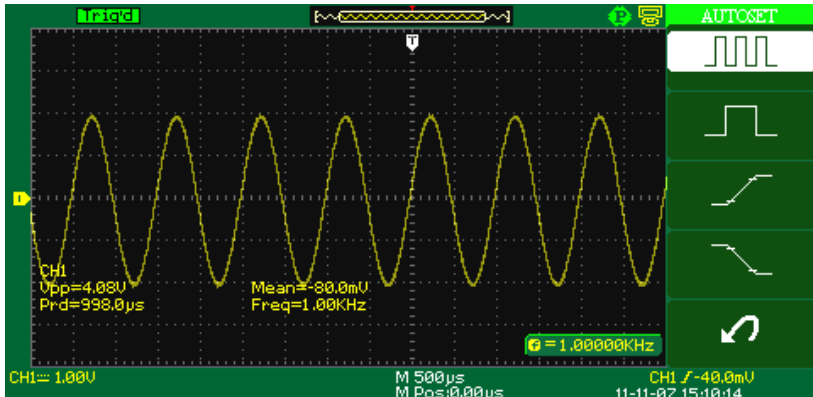
Figure 13 - Auto Setup
