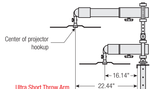
Ultra Short Throw Arm
