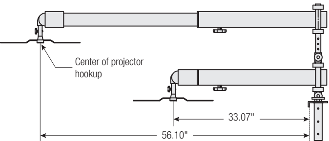
Short Throw Arm
