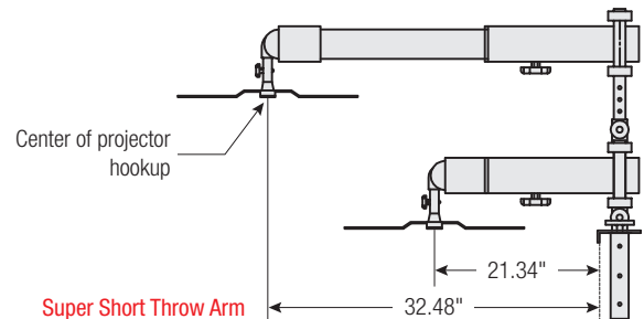
Super Short Throw Arm
