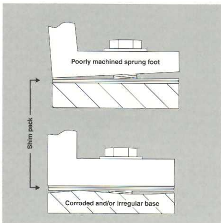
Typical problems that can be solved with Sof' Shoe shim.
