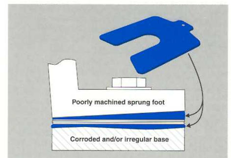
Sof' Shoe shims added to both sides of the shim pack "cold flow" to fill irregular gaps.
