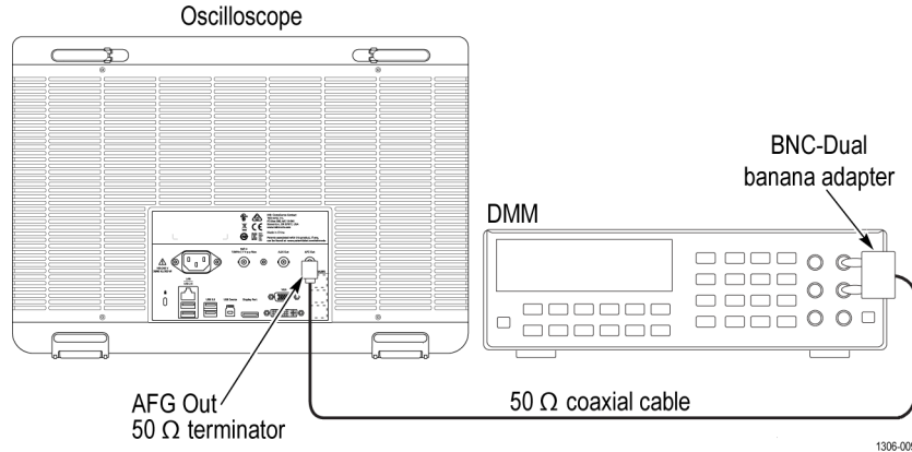
Figure 4: Amplitude test
