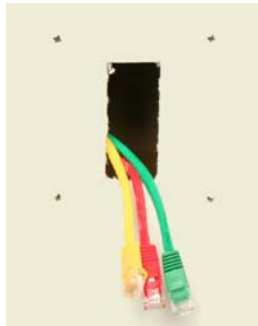
Fig.8: The three Cat-5e cables have been installed and pulled through the rectangular opening in the wall.
