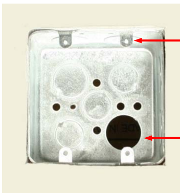
Fig.5: Conduit knock-out removed
