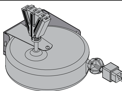
Universal Cord Reel Kit 15' [457.2 cm] retractable, 12 AWG, with breaker, includes universal mounting bracket (mounts horizontally or vertically inside lectern to base panel) 10 lbs [.45 kg] 99037
