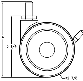
3" Twin-Wheel caster (TW)
