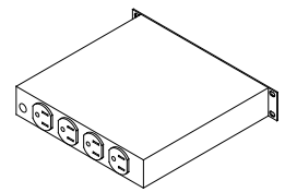
1/2 Rack 4-Outlet Power Strip 15-amp (1RU) 10.375"W x 7.1875"D x 1.75"H 97013
