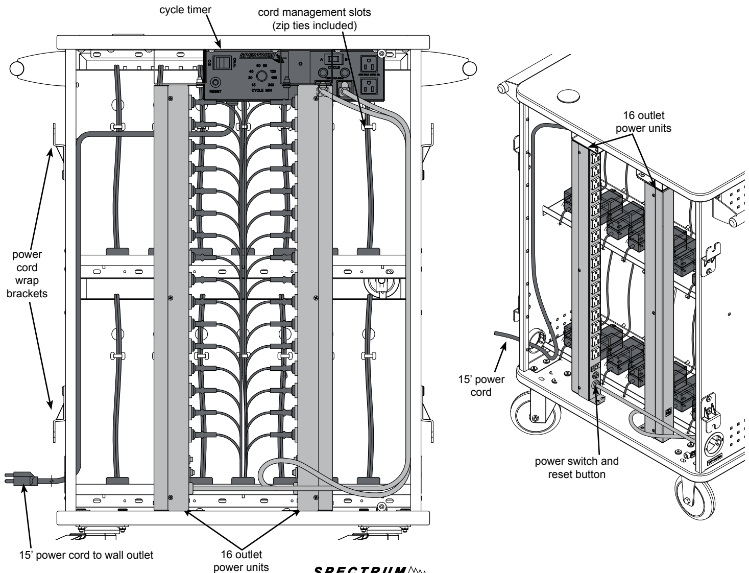
electrical side views (shown with door removed)
