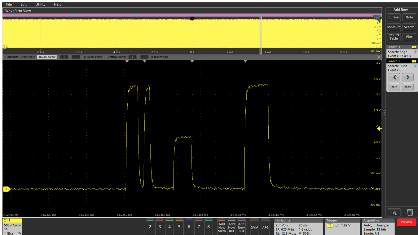
Figure 21: Earlier, FastAcq revealed the presence of a runt pulse in a digital data stream prompting further investigation. In this long 20 ms acquisition, Search 1 reveals that there are approximately 37,500 rising edges in the acquisition. Search 2 (run simultaneously) reveals that there are six runt pulses in the acquisition.
