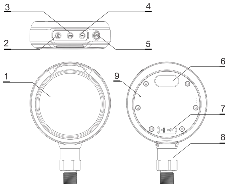
Figure 1 Basic Structure
