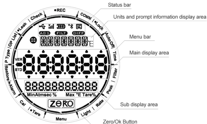
Figure 2 Main Display
