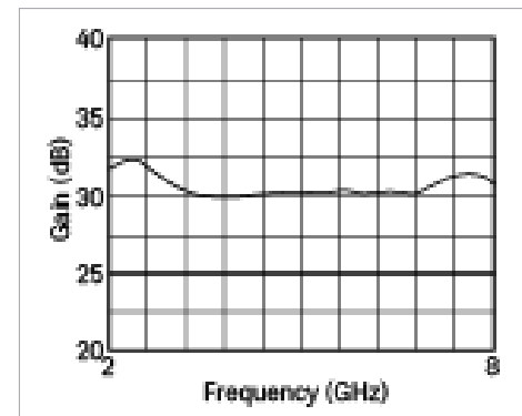
Figure 3. Gain vs. Frequency
