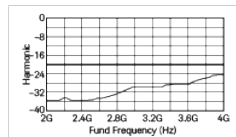
Figure 4. Harmonics vs. Frequency
