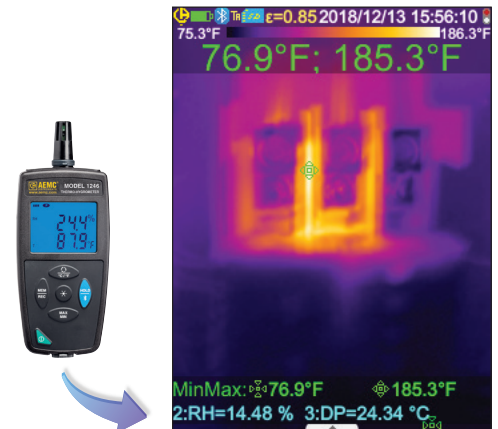
Thermogram and connectivity to the Thermo-Hygrometer Model 1246
