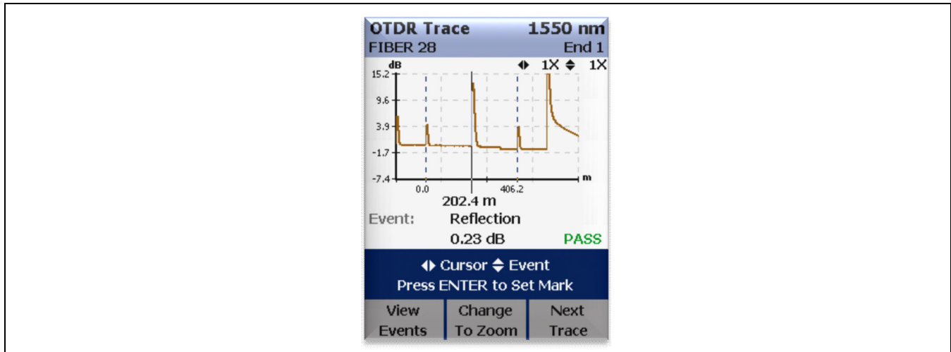
Figure 10: OTDR Trace Example
