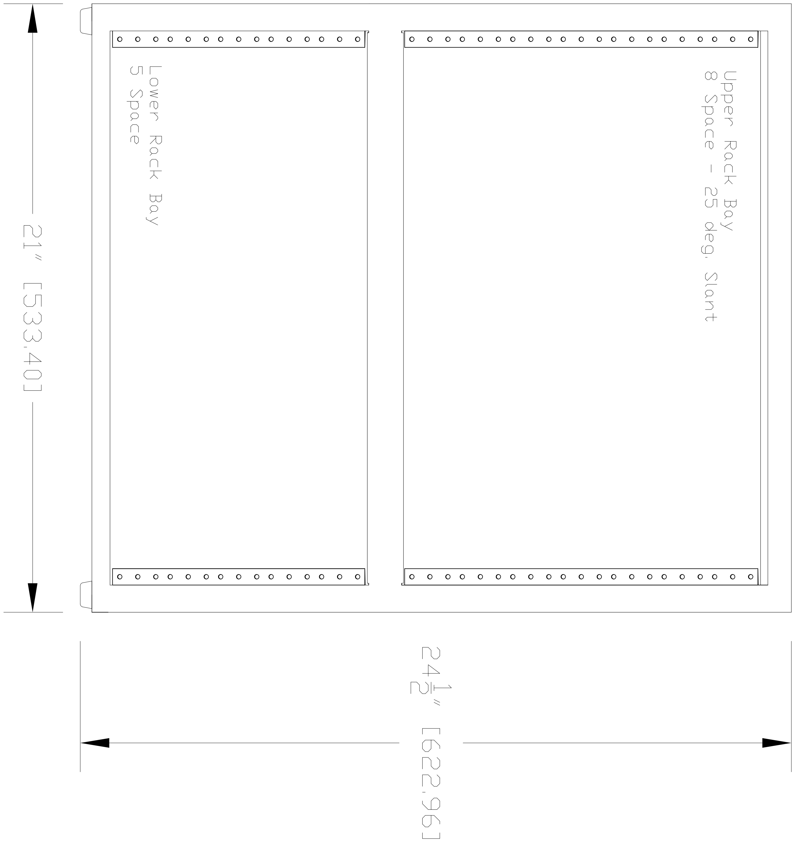
FRONT VIEW
