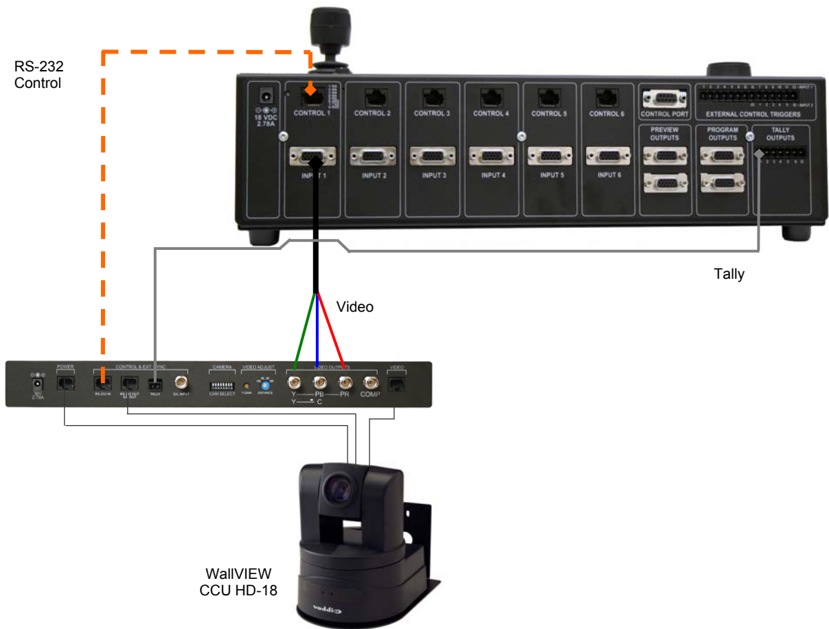
Figure 6: Sample configuration of a WallVIEW CCU connected to ProductionVIEW HD, with video, control and tally cabling.
