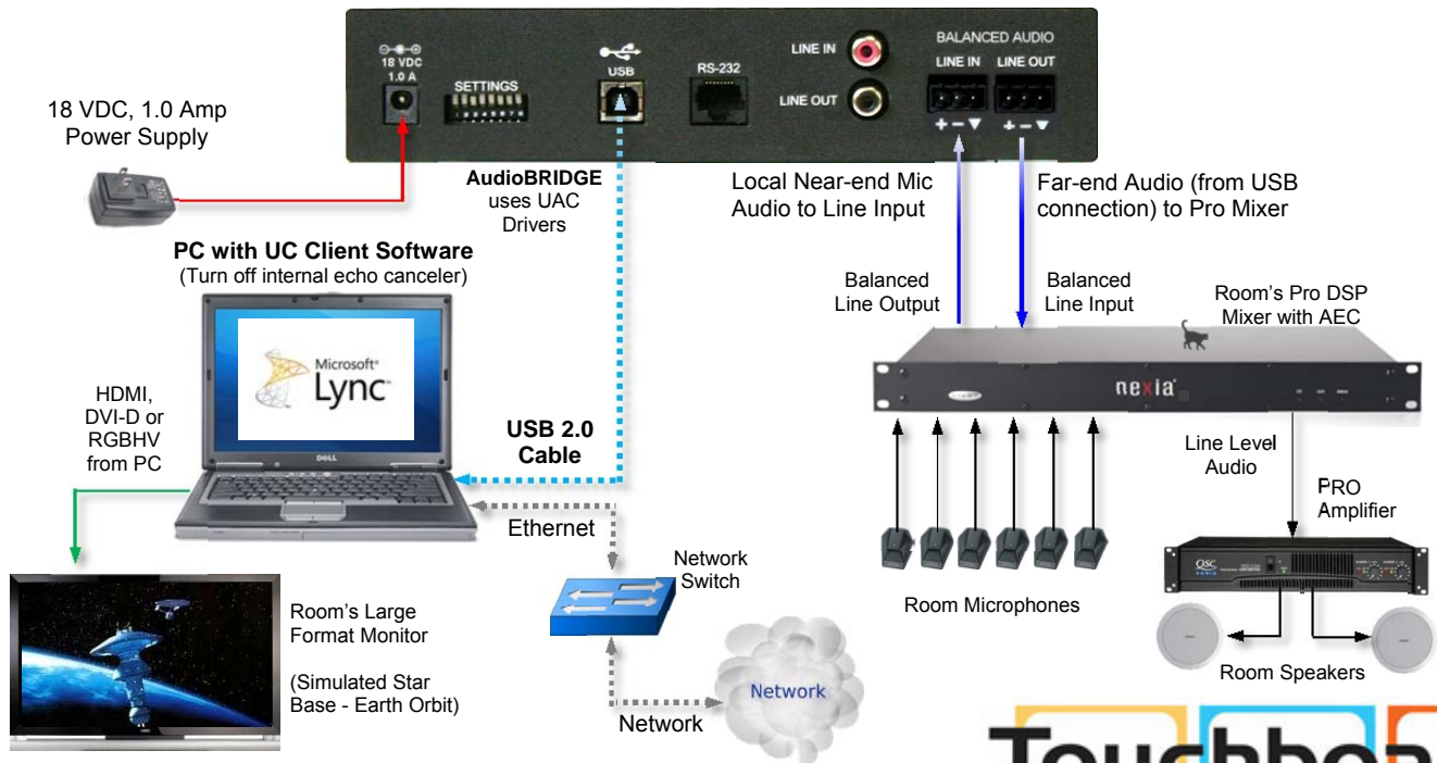
EasyUSB AudioBRIDGE - Rear Panel Connections
