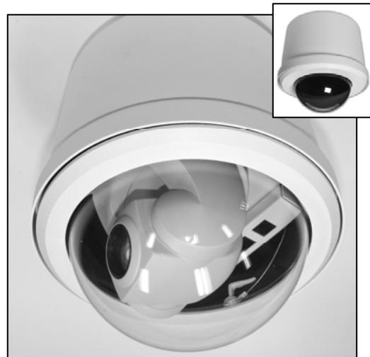
Figure 1: DomeVIEW Indoor Pendant Mount Dome System shown with Sony EVI-D70 PTZ camera and EZCamera Cabling Shoe mounted in the enclosure (Upper Right: Indoor Pendant Dome shown with smoke tinted bubble - clear is standard).
