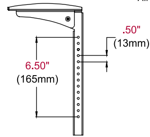
BRACKET DETAIL
